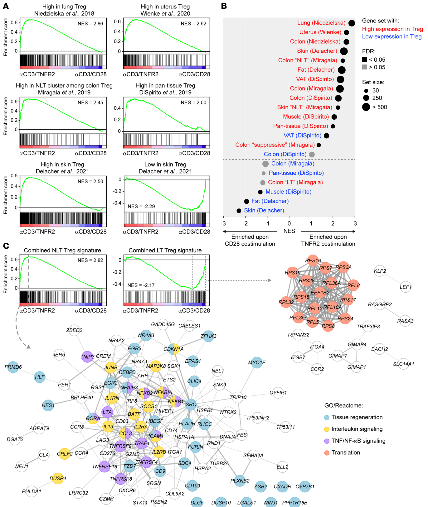
Figure 6. Enrichment of healthy NLT Treg gene signatures in TNFR2-costimulated tTregs. (A) GSEA plots showing enrichment of indicated published Treg gene signatures from healthy tissues and peripheral blood (40, 46–49) in the transcriptomes of tTregs costimulated via TNFR2 or CD28 for 7 days. Normalized enrichment scores (NES) are depicted (FDR < 0.05). (B) Summary of GSEA data showing enrichment of published Treg gene signatures in healthy tissues (40, 46–49) in the transcriptome of TNFR2- or CD28-costimulated tTregs. Red and blue text mark gene sets describing, respectively, high and low expression in Tregs from indicated tissues. The first author of the corresponding reference is shown between parentheses. Additional information
